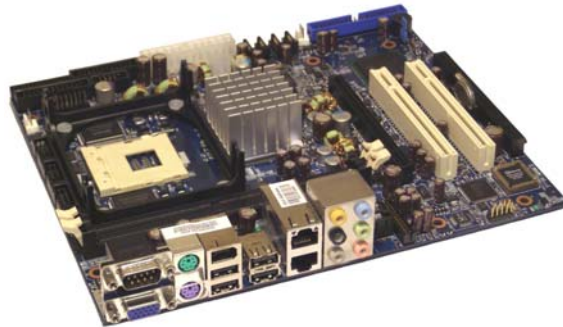
986LCD-M/Flex
